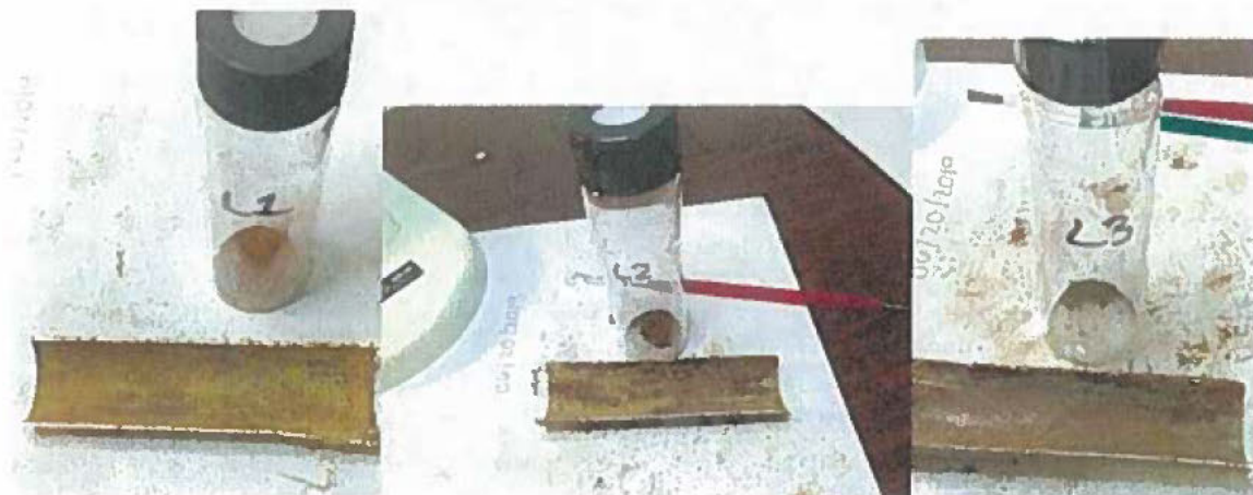
Figure 4-13 Layers of Scale Removed from Harvested Pipe
