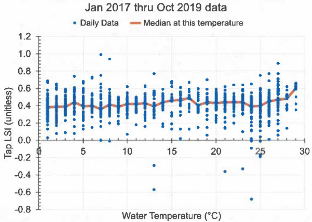
Figure 4 Daily and median LSI data calculated on dates from Jan 2017 through October 2019 with the same temperature
