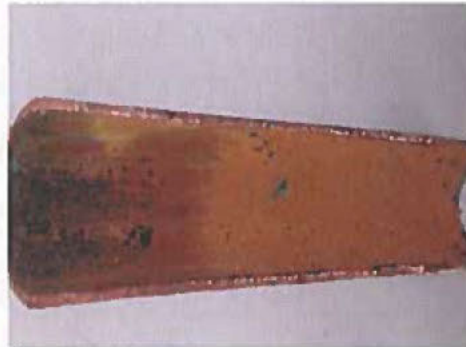
Figure 4-12 Pipe Prior to Scale Removal
