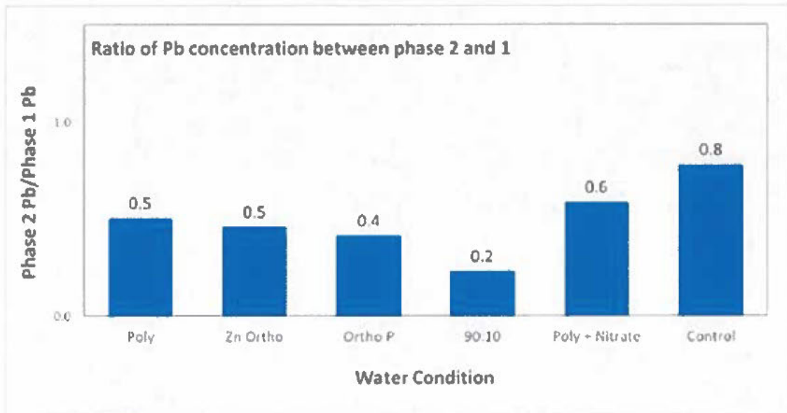
Figure 4-25 Relative Lead Leaching Under More Corrosive Conditions of Phase 2 (2/3 Kankakee and 1/3 Synthesized Water) Divided by Results of Phase 1 (100% Kankakee)
