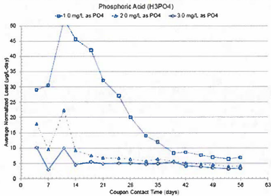
Figure 4-3 Summer/Fall 2019 Average Lead Solubility Test Results (Two Replicates) – H 3 PO 4 Phosphate (Sep-Nov 2019)
