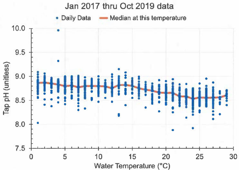
Figure 5 Daily and median pH data measured on dates from Jan 2017 through October 2019 with the same temperature
