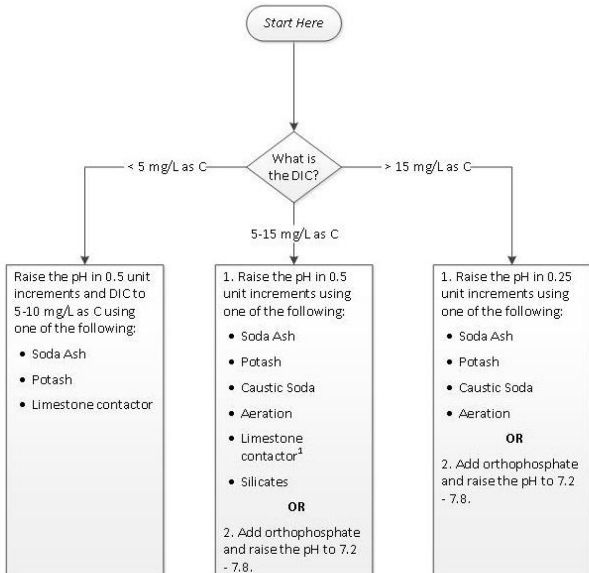
Flowchart 1a: Selecting Treatment for Lead only or Lead and Copper with pH < 7.2
