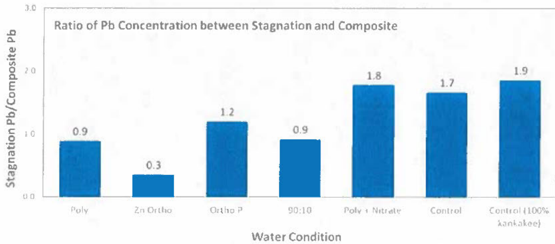
Figure 4-26 Relative Level of Lead Under Long Stagnation Times (72-96 hours) Versus That Obtained During 24 Hour Composite Sampling (24 Hours)
