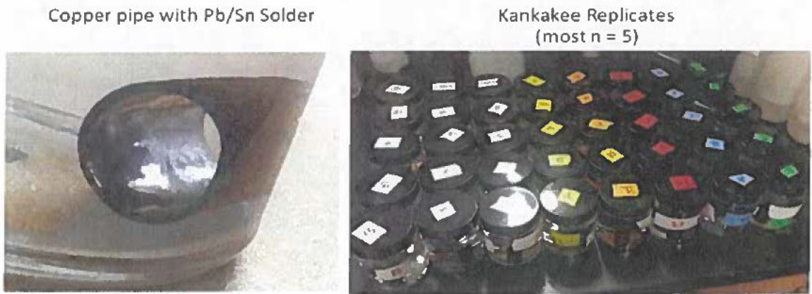
Figure 4-21 Apparatus Used for Testing. Solder Coupons in Glass Jars (Left) and 5 Replicates for Each Inhibitor Condition (Right)
