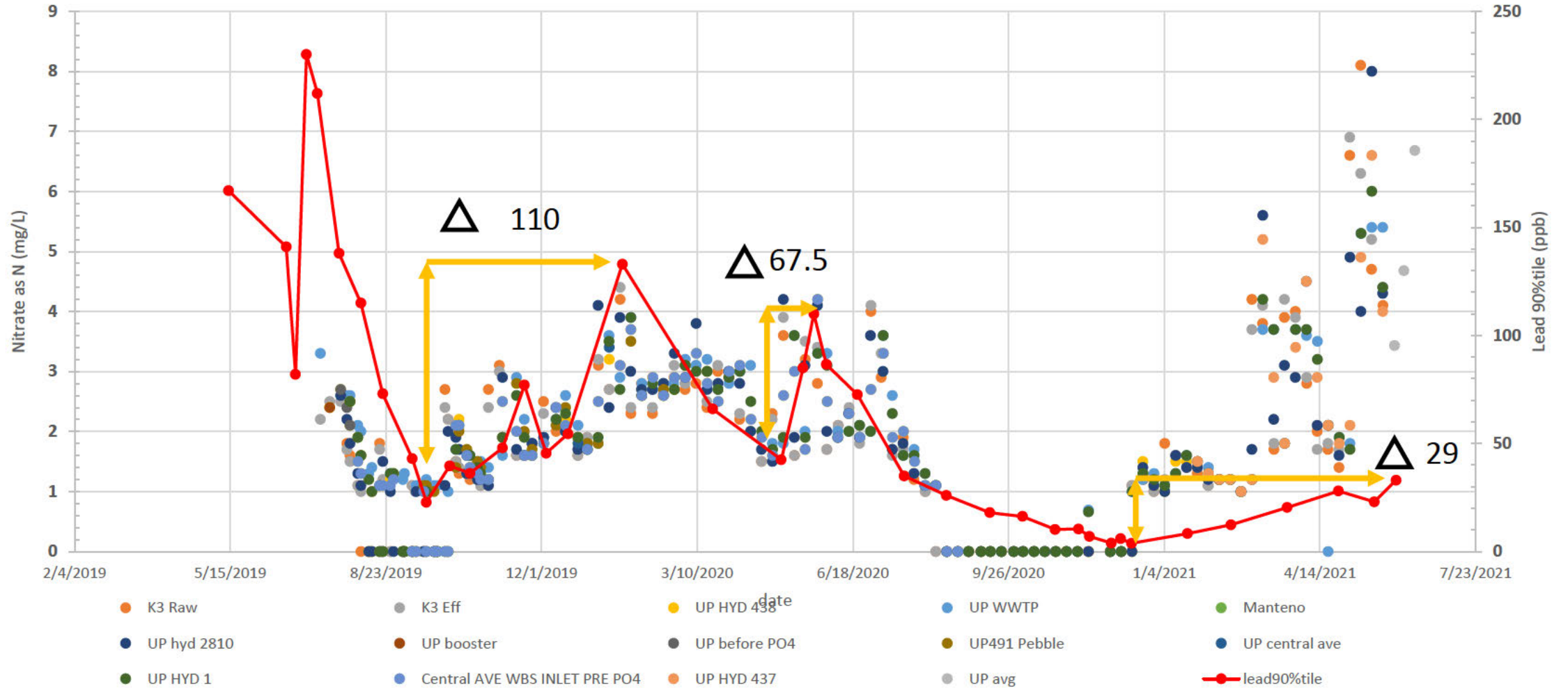
Lead 90%tile vs. Nitrate
