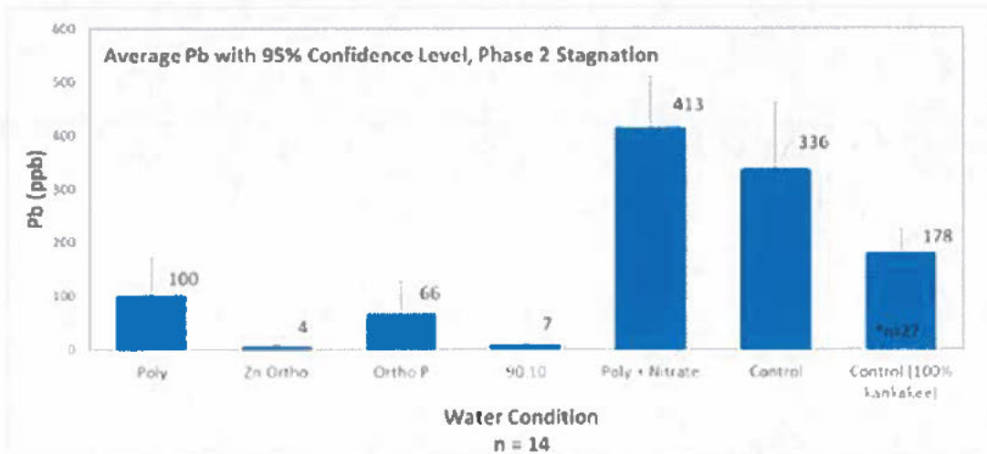
Figure 4-27 Results with 95% Confidence Intervals for Samples Collected with Either 72 or 96 Hours Stagnation
