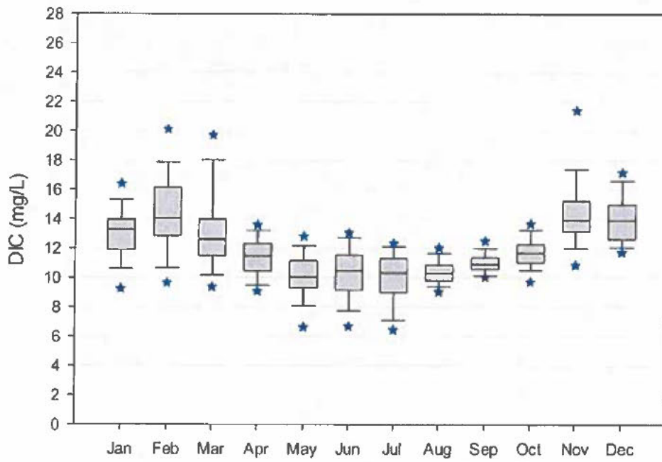
Figure 2-8 Source Water (Kankakee Tap) – Calculated Monthly Dissolved Inorganic Carbon (DIC) – Jan 2017-Oct 2019
