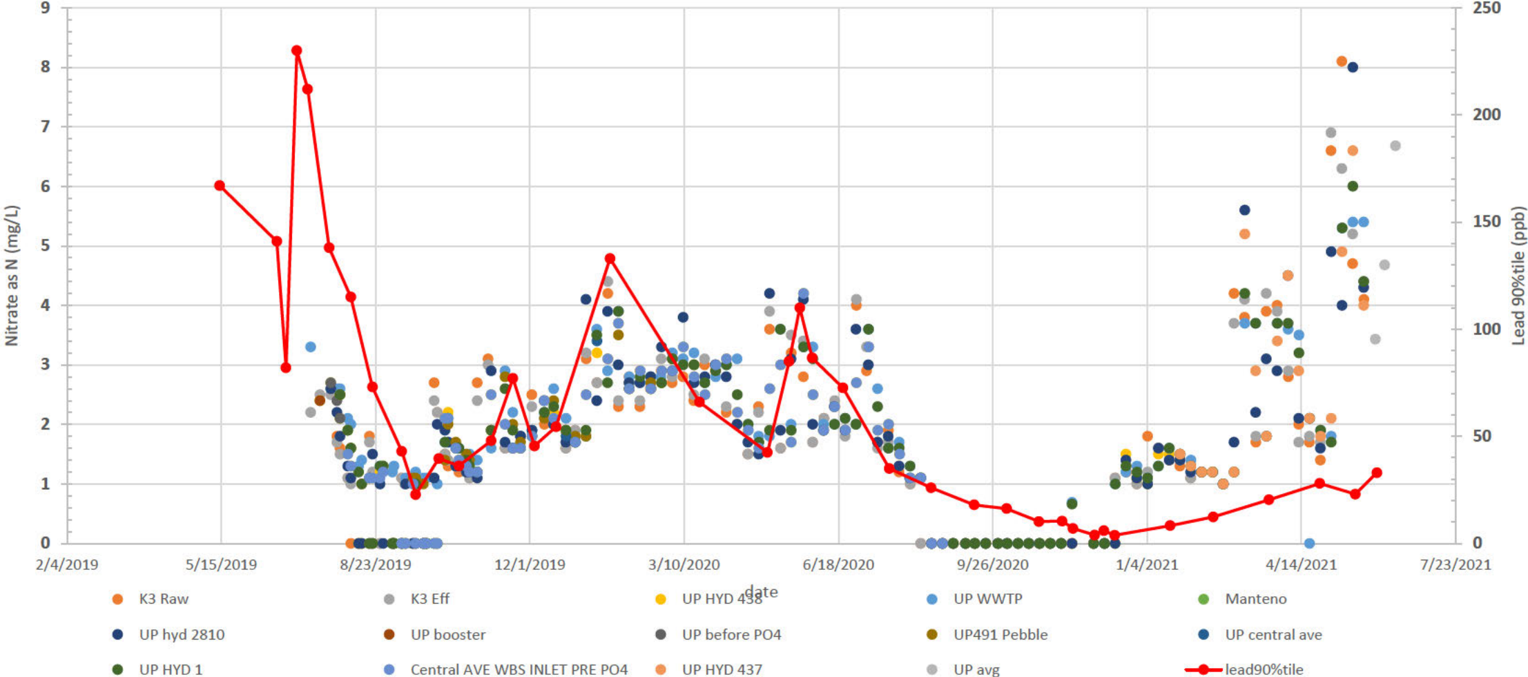
Lead 90%tile vs. Nitrate
