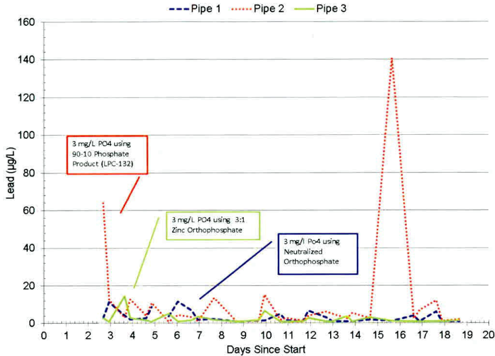
Figure 5 Lead solubility dump/fill studies with harvested pipe comparing 3 mg/L as PO 4 doses of a 90/10 ortho/poly blend, ZOP, and neutralized orthophosphate (NaH 2 PO 4 )
