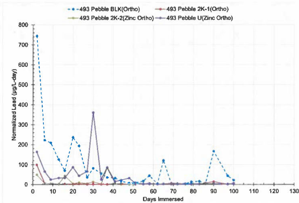
Figure 12 Four segments of household plumbing harvested from one UP house, treated with 3 mg/L as PO 4 dose, with either ZOP or H 3 PO 4 – 0 to 800 µg/L-day scale
