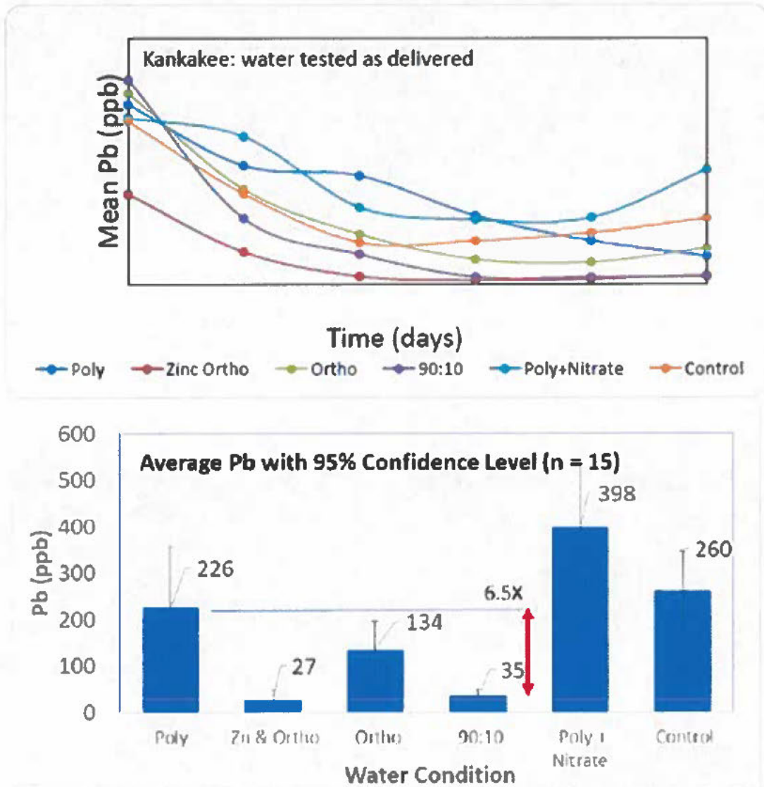
Figure 4-23 Results of Composite Samples from All Replicates, Indicating Trends in Lead Release Using 100% Kankakee Water with Different Types of Corrosion Control (Upper) During the last three days of sampling, each of the five replicates was sampled on three sequential days (n=15) to create final results with 95% confidence intervals (lower).
